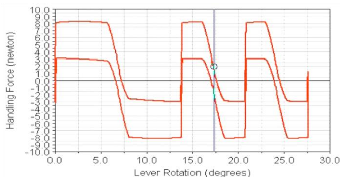
Picture 3 Simulated handling force vs gear stick rotation which correlates extremely well with the real world after using ForceBoard to measure the exact coefficient of friction between plunger and index track.
